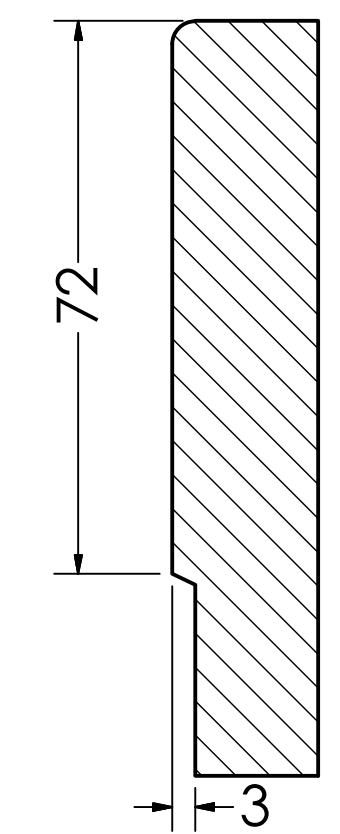
SECTION A SCALE 1 / 25
